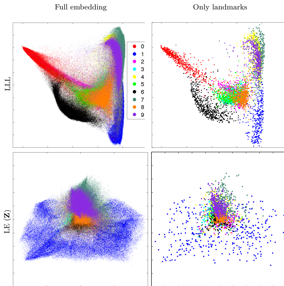
Fig. 7. Embedding of 1020000 points from the infinite MNIST dataset using 10000 landmarks. Top: LLL, bottom: LE ( \mathbf{Z} ). Left: full dataset \mathbf{X} , right: landmarks \tilde{\mathbf{X}} only.
